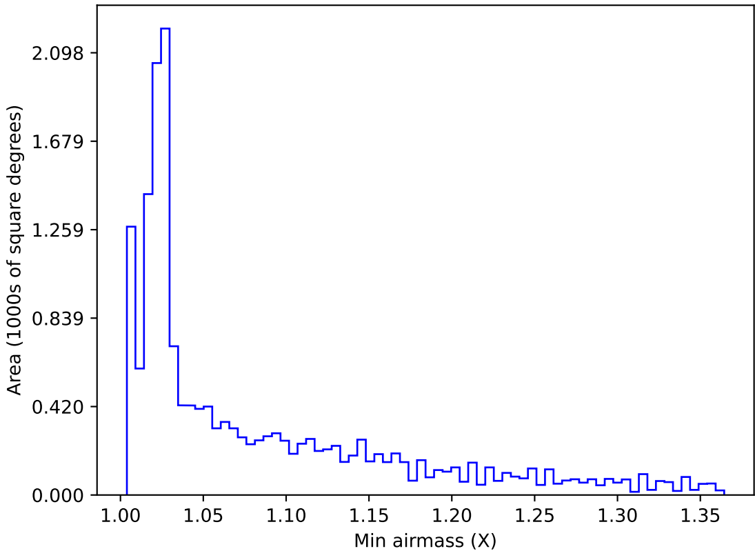
too_elab_r256_d2_gz_v3.4_10yrs WFD all bands: Min airmass
