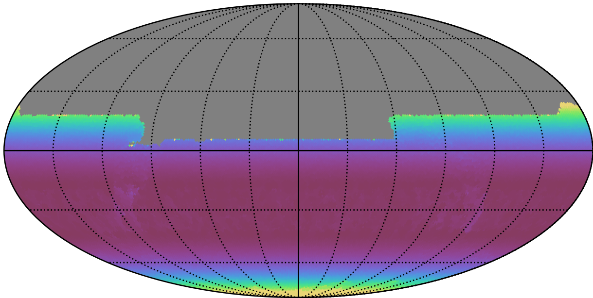
too_elab_r256_d2_gz_v3.4_10yrs All sky y band: Min airmass
