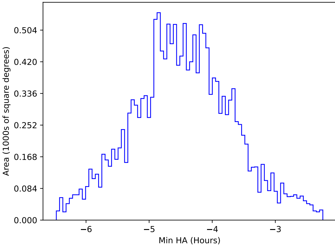
too_elab_r256_d2_gz_v3.4_10yrs WFD z band: Min HA
