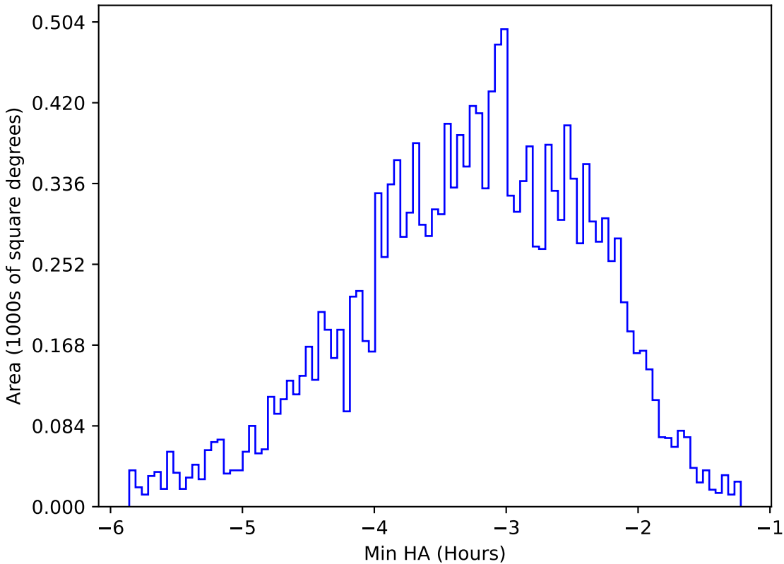
too_elab_r256_d2_gz_v3.4_10yrs WFD u band: Min HA
