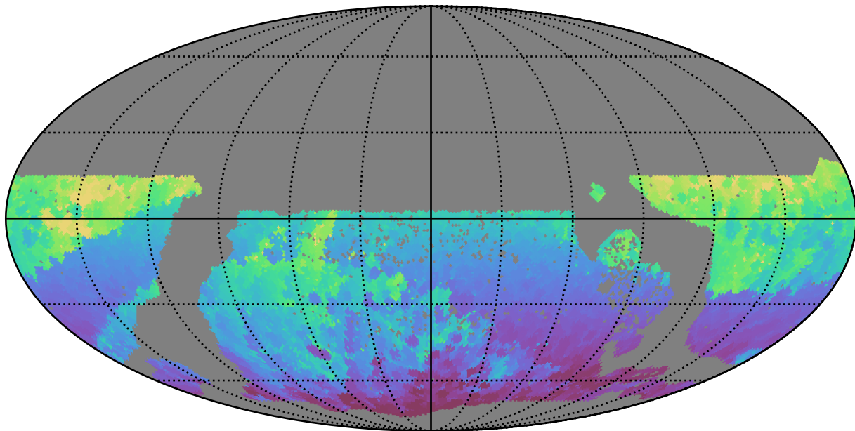
too_elab_r256_d2_gz_v3.4_10yrs WFD r band: Min HA
