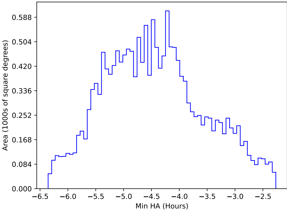
too_elab_r256_d2_gz_v3.4_10yrs WFD r band: Min HA
