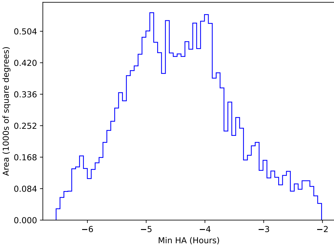
too_elab_r256_d2_gz_v3.4_10yrs WFD i band: Min HA
