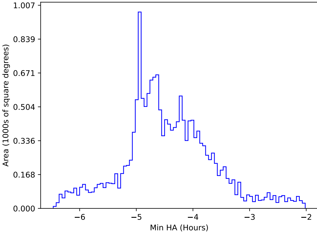
too_elab_r256_d2_gz_v3.4_10yrs WFD g band: Min HA
