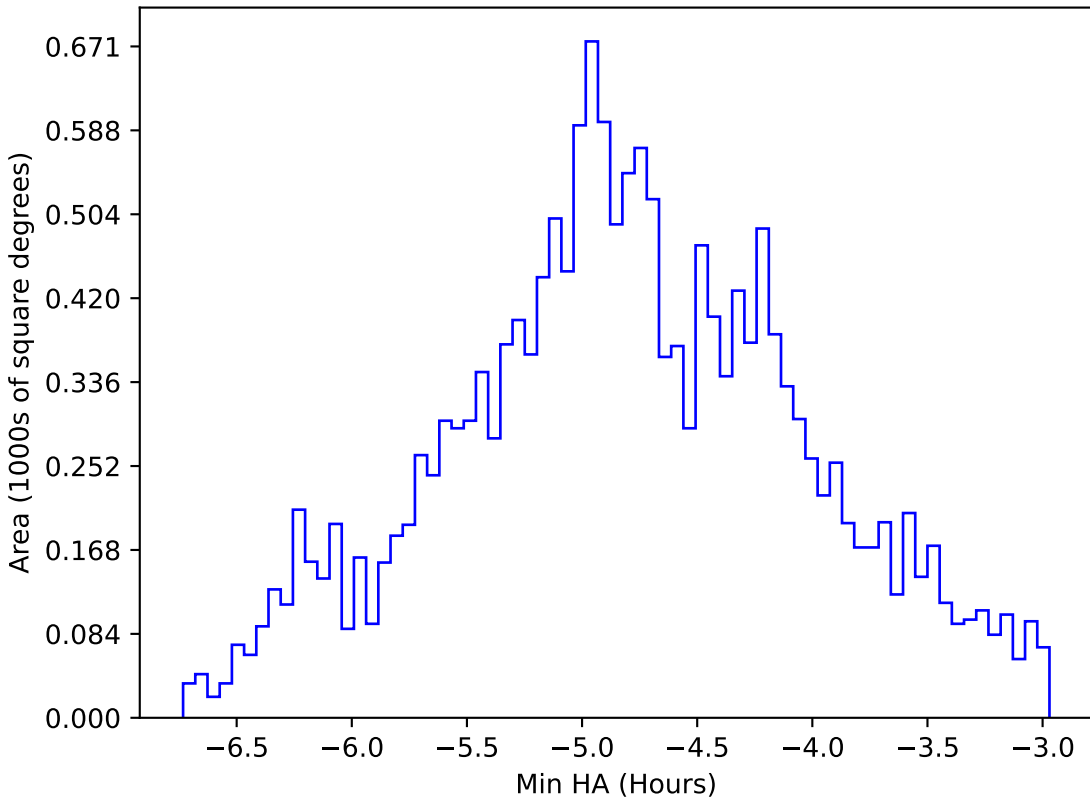
too_elab_r256_d2_gz_v3.4_10yrs WFD all bands: Min HA
