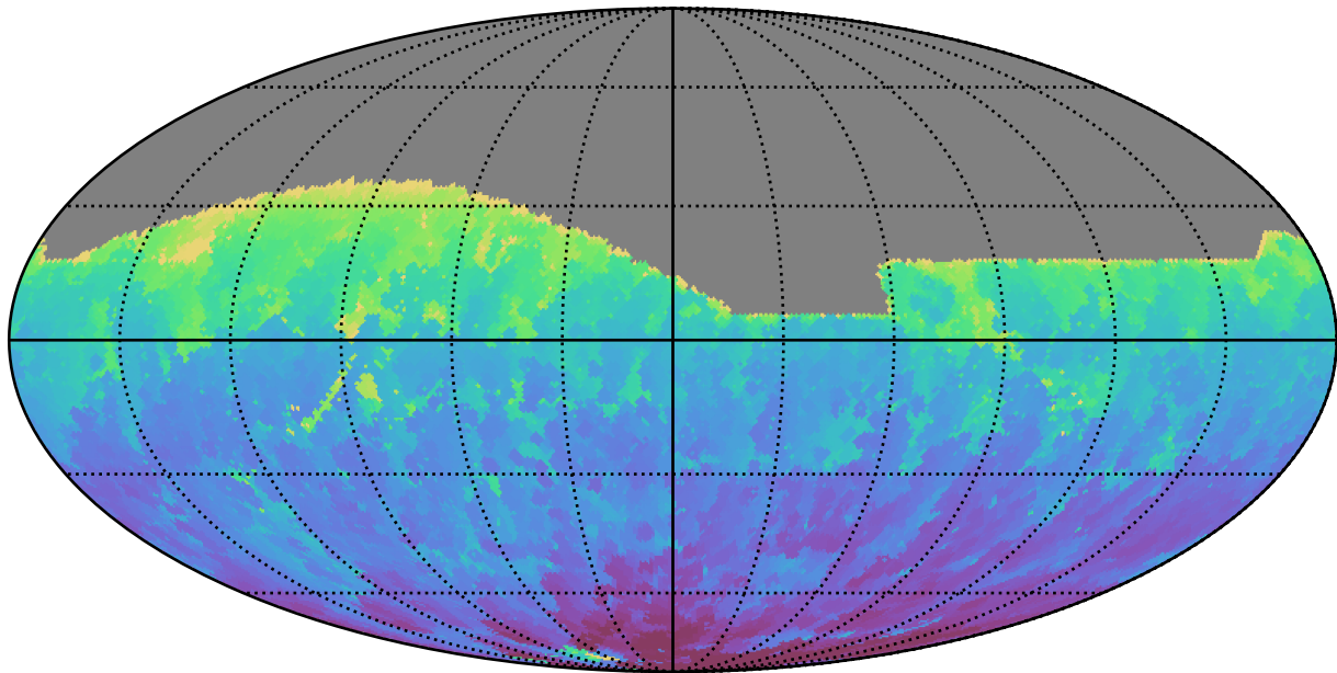
too_elab_r256_d2_gz_v3.4_10yrs All sky z band: Min HA
