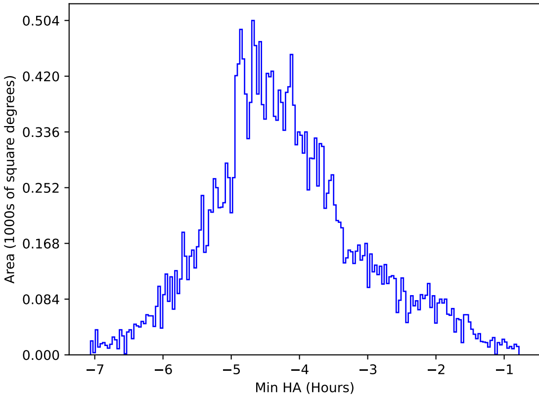
too_elab_r256_d2_gz_v3.4_10yrs All sky z band: Min HA
