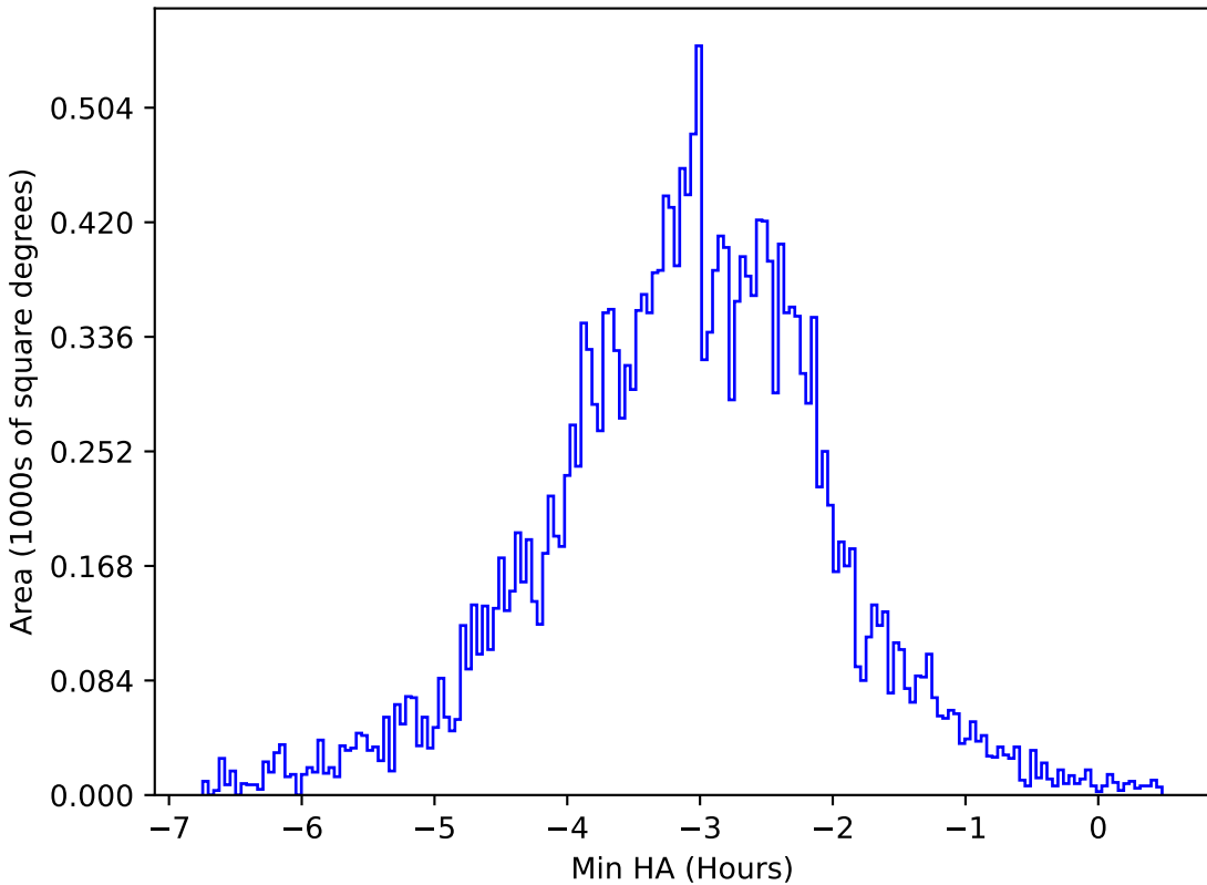
too_elab_r256_d2_gz_v3.4_10yrs All sky u band: Min HA
