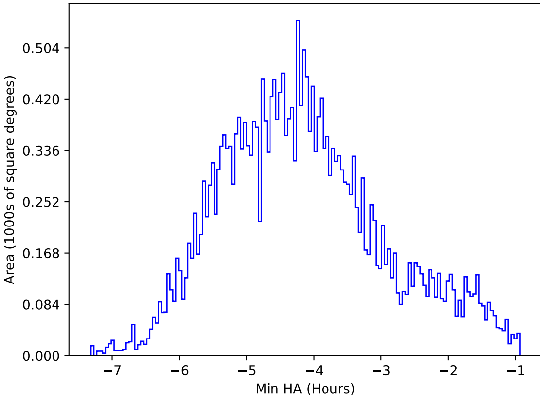
too_elab_r256_d2_gz_v3.4_10yrs All sky r band: Min HA
