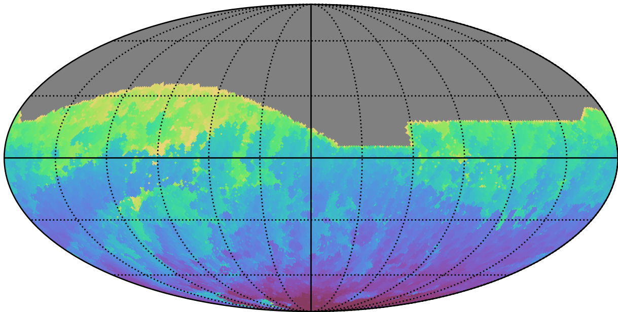
too_elab_r256_d2_gz_v3.4_10yrs All sky i band: Min HA
