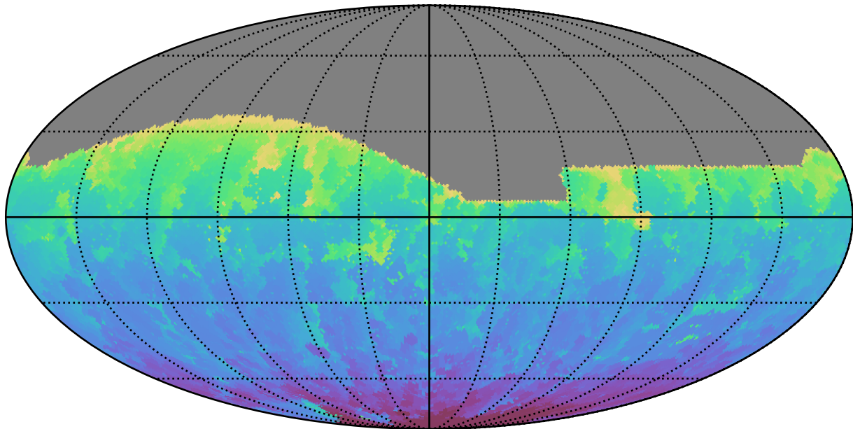
too_elab_r256_d2_gz_v3.4_10yrs All sky g band: Min HA
