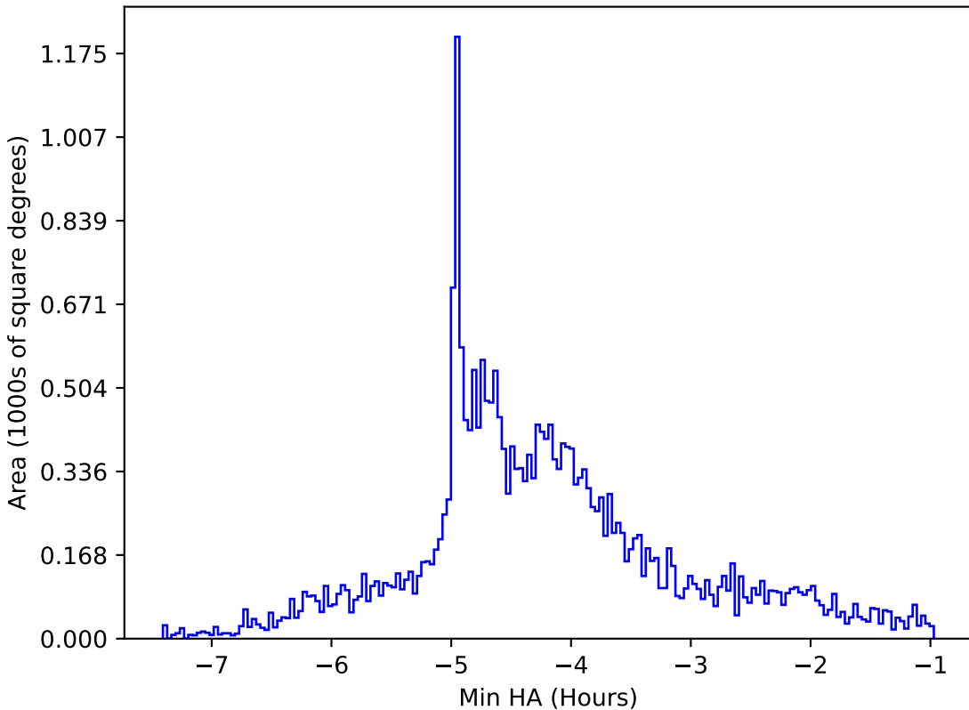
too_elab_r256_d2_gz_v3.4_10yrs All sky g band: Min HA
