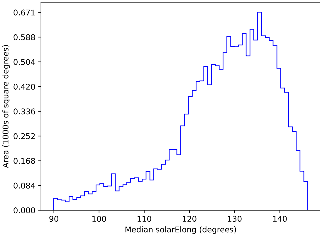
too_elab_r256_d2_gz_v3.4_10yrs WFD z band: Median solarElong
