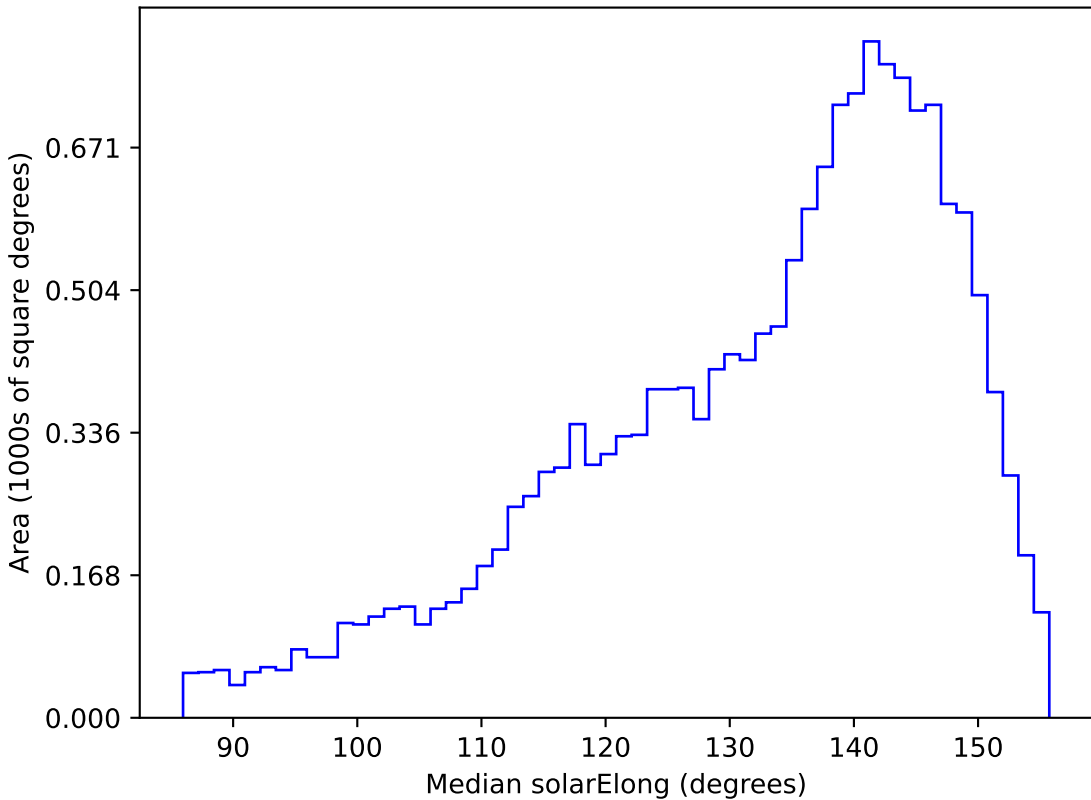
too_elab_r256_d2_gz_v3.4_10yrs WFD u band: Median solarElong
