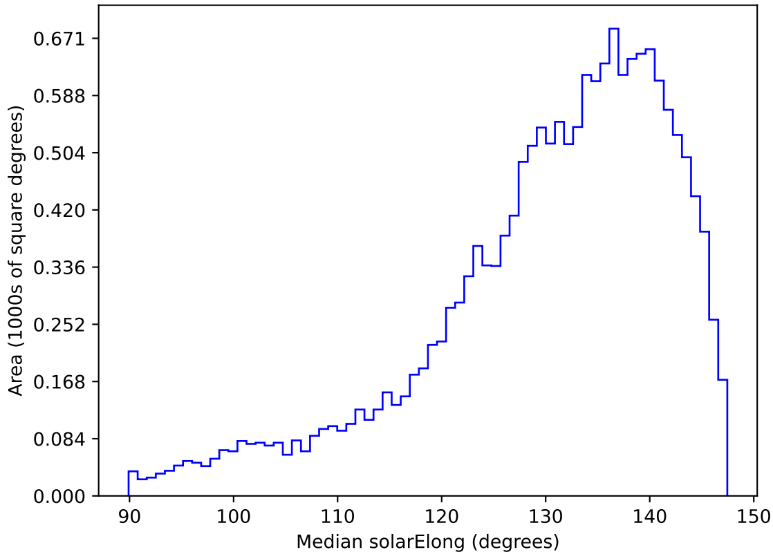
too_elab_r256_d2_gz_v3.4_10yrs WFD r band: Median solarElong
