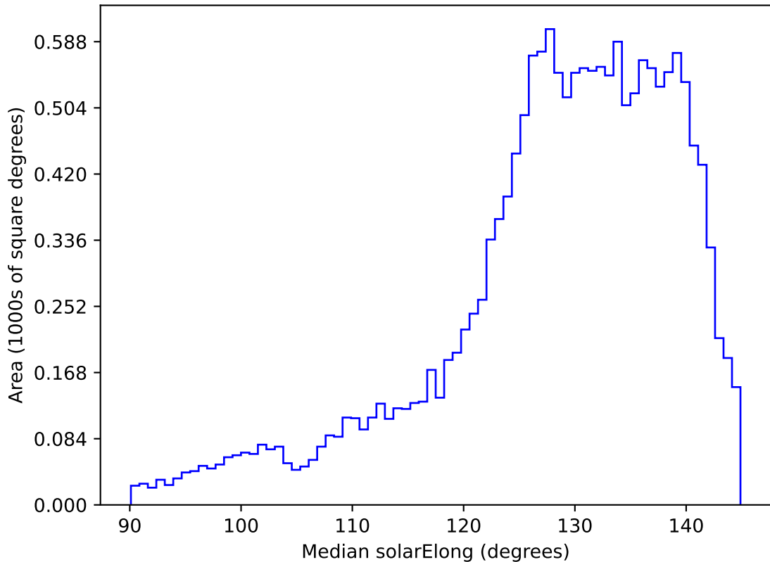
too_elab_r256_d2_gz_v3.4_10yrs WFD i band: Median solarElong
