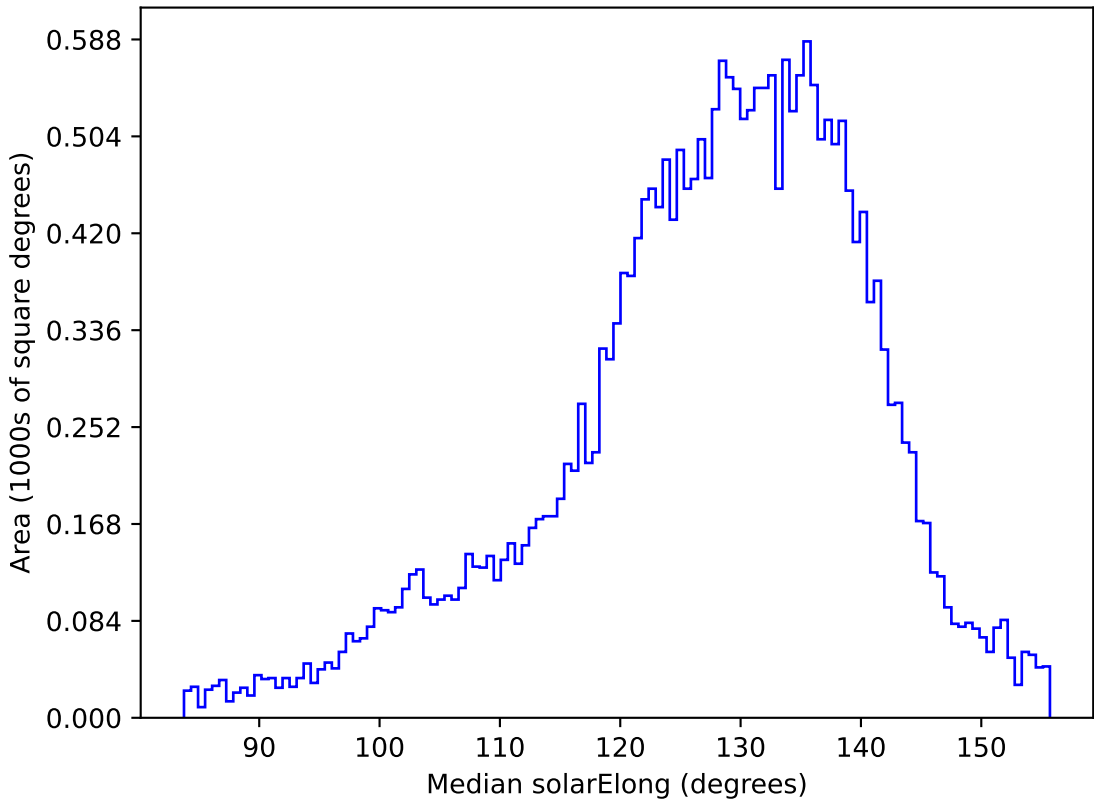
too_elab_r256_d2_gz_v3.4_10yrs All sky z band: Median solarElong
