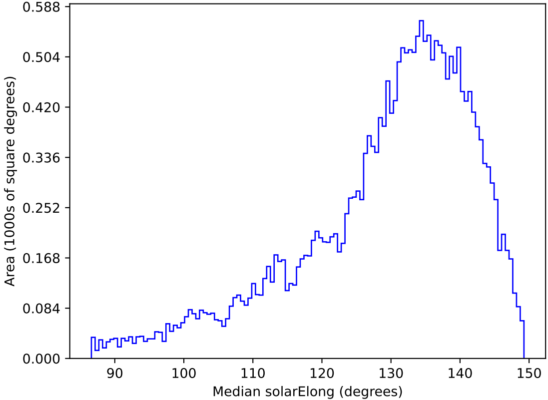
too_elab_r256_d2_gz_v3.4_10yrs All sky y band: Median solarElong
