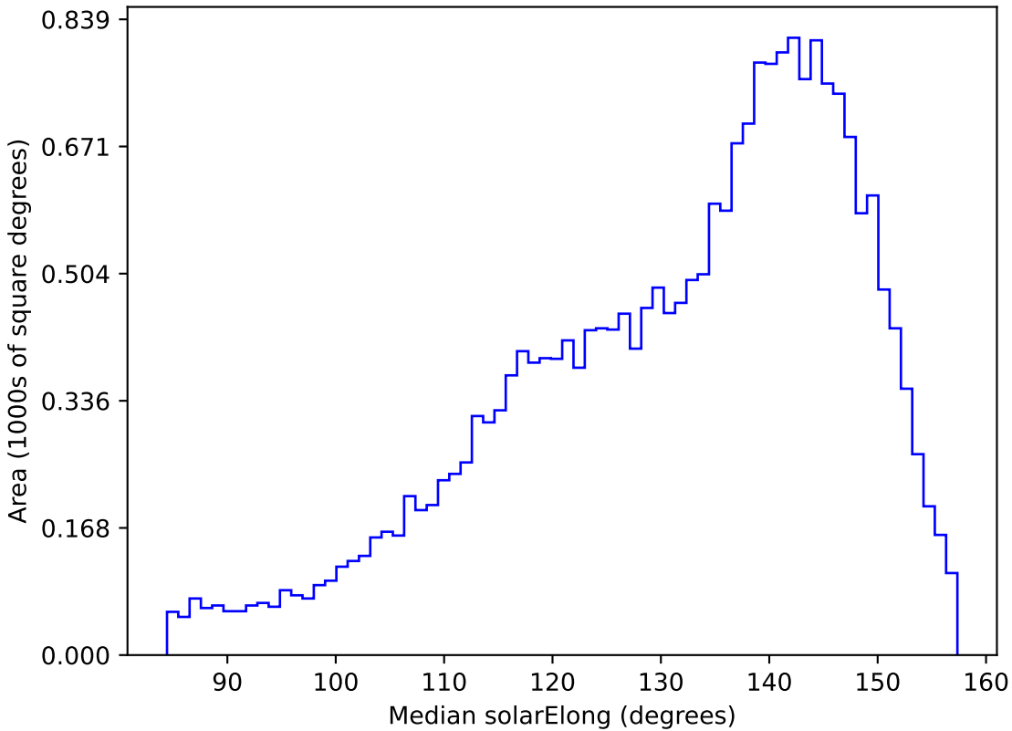
too_elab_r256_d2_gz_v3.4_10yrs All sky u band: Median solarElong
