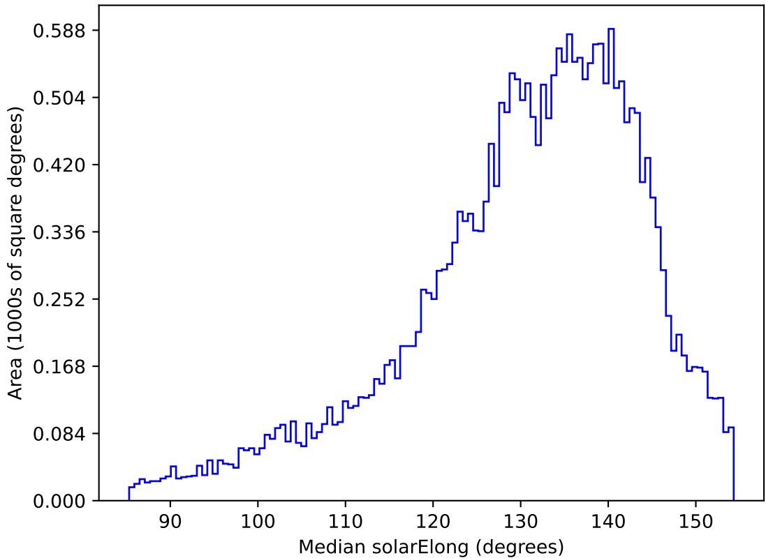
too_elab_r256_d2_gz_v3.4_10yrs All sky r band: Median solarElong
