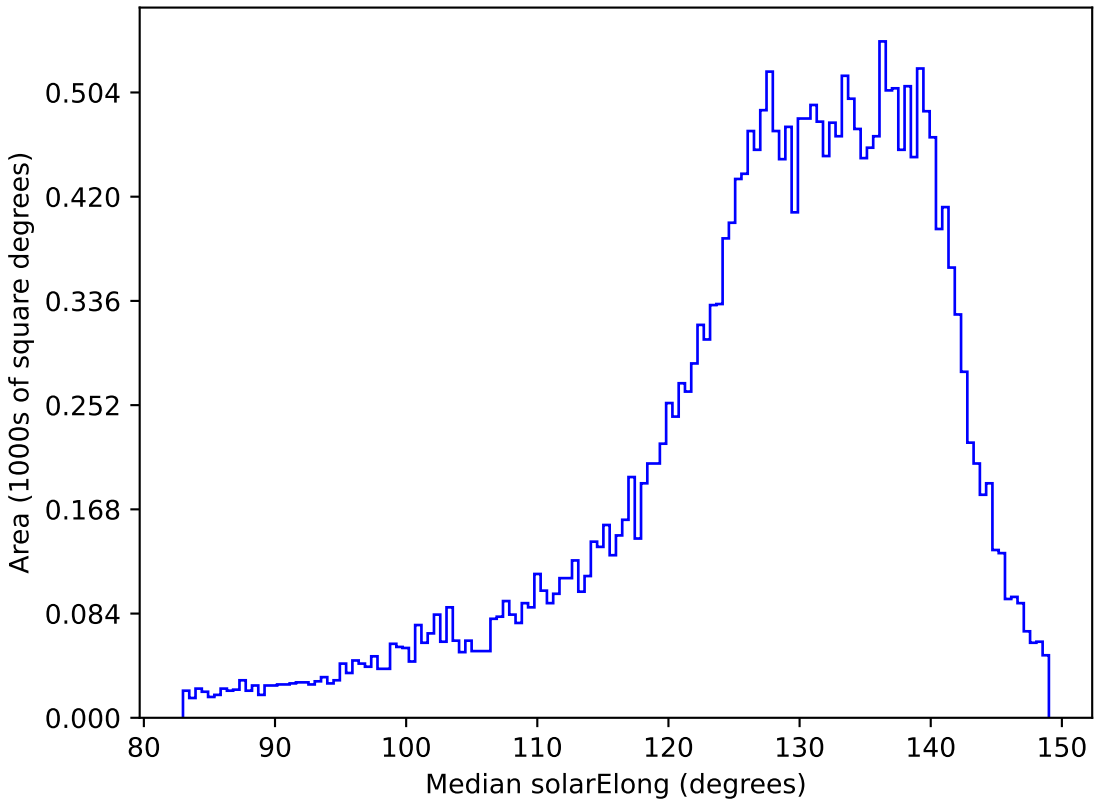
too_elab_r256_d2_gz_v3.4_10yrs All sky i band: Median solarElong
