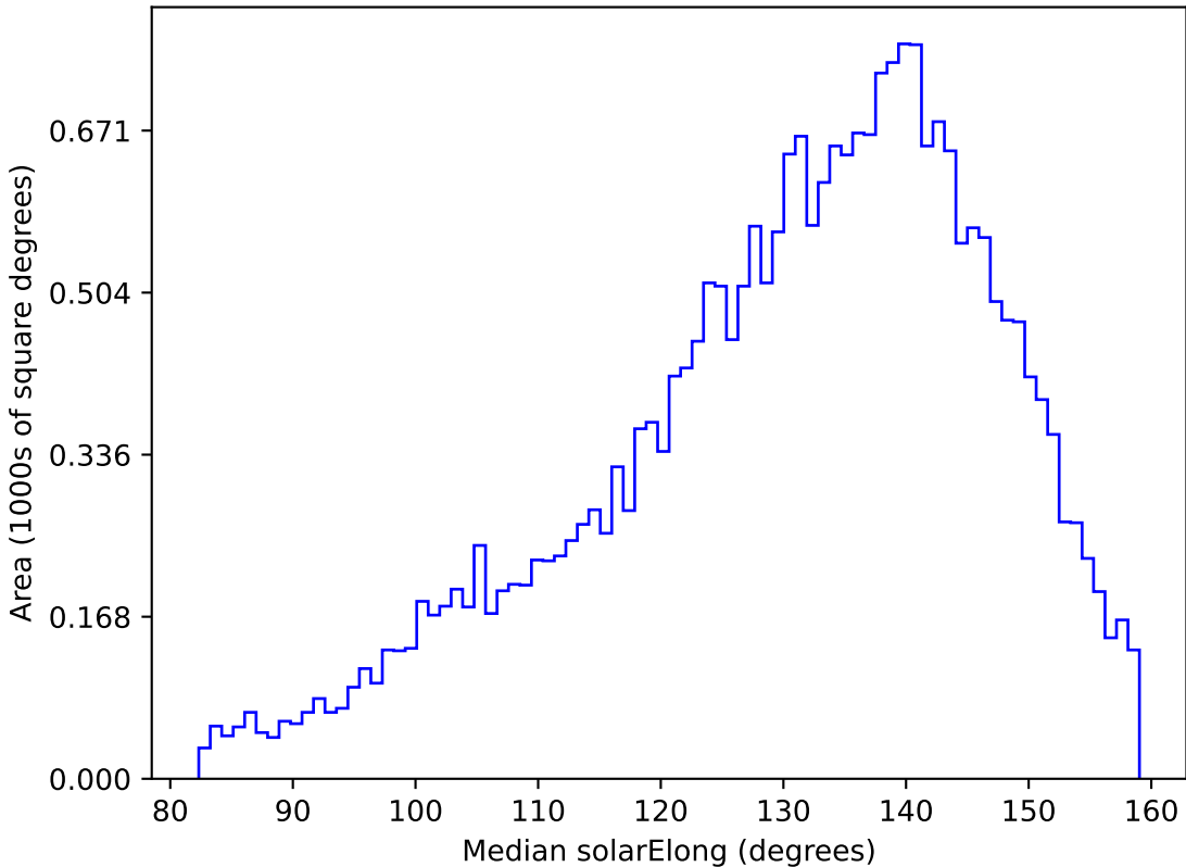
too_elab_r256_d2_gz_v3.4_10yrs All sky g band: Median solarElong
