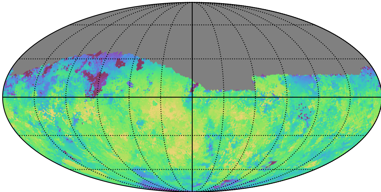
too_elab_r256_d2_gz_v3.4_10yrs Yr 1 z band: Median skyBrightness
