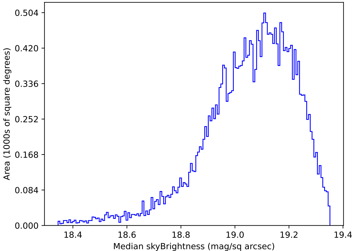
too_elab_r256_d2_gz_v3.4_10yrs Yr 1 z band: Median skyBrightness
