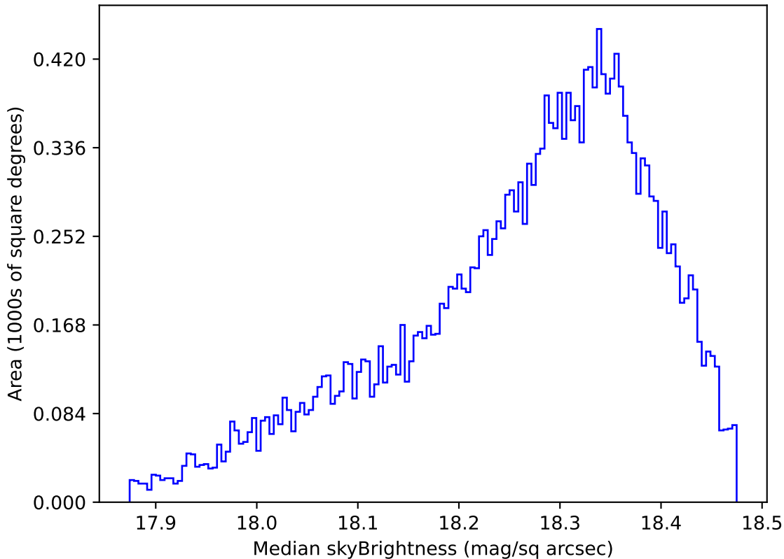
too_elab_r256_d2_gz_v3.4_10yrs Yr 1 y band: Median skyBrightness
