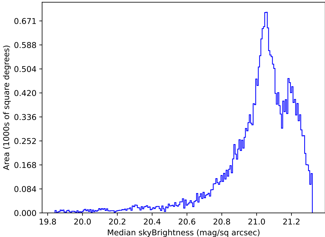
too_elab_r256_d2_gz_v3.4_10yrs Yr 1 r band: Median skyBrightness
