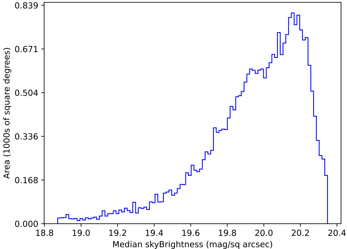
too_elab_r256_d2_gz_v3.4_10yrs Yr 1 i band: Median skyBrightness
