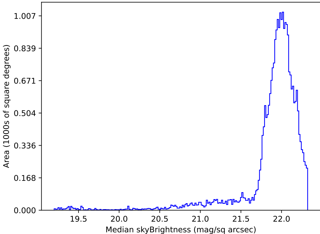
too_elab_r256_d2_gz_v3.4_10yrs Yr 1 g band: Median skyBrightness
