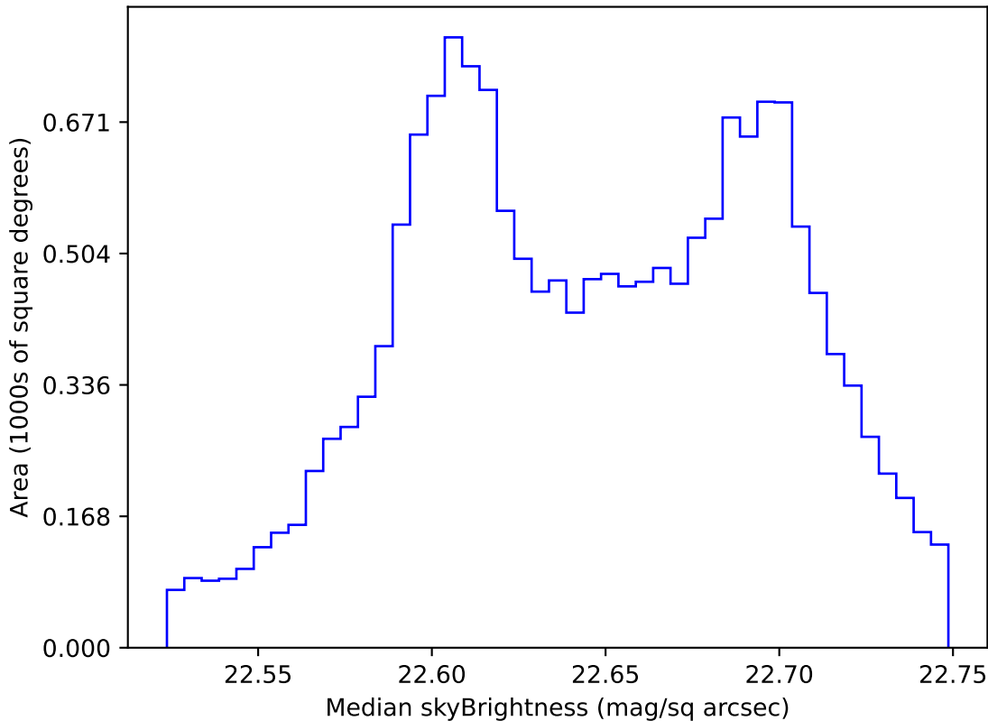
too_elab_r256_d2_gz_v3.4_10yrs WFD u band: Median skyBrightness
