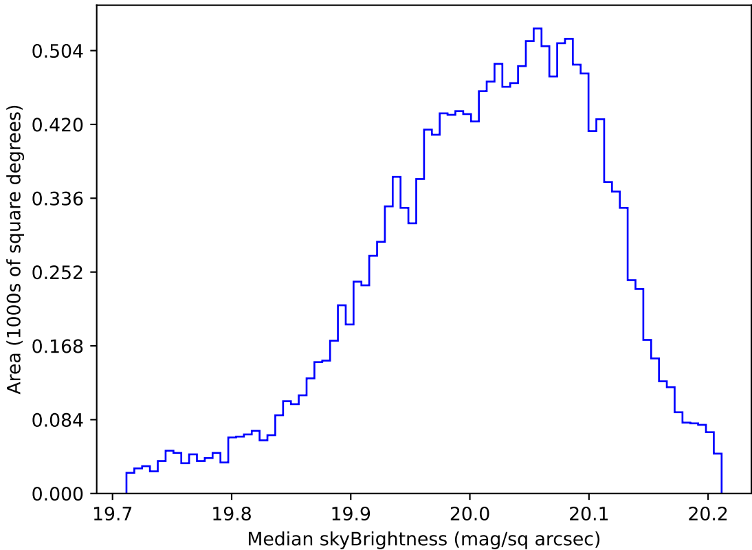
too_elab_r256_d2_gz_v3.4_10yrs WFD i band: Median skyBrightness
