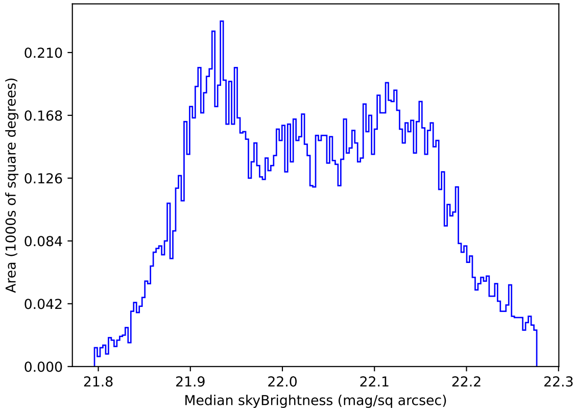
too_elab_r256_d2_gz_v3.4_10yrs WFD g band: Median skyBrightness
