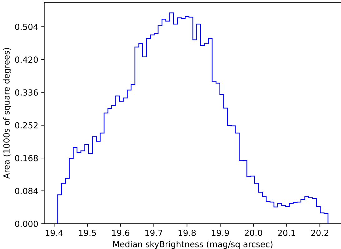
too_elab_r256_d2_gz_v3.4_10yrs WFD all bands: Median skyBrightness
