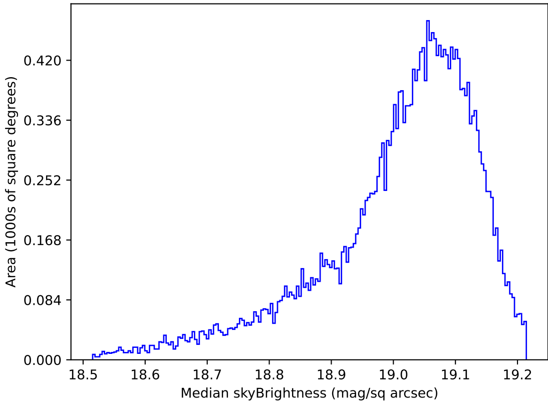
too_elab_r256_d2_gz_v3.4_10yrs All sky z band: Median skyBrightness
