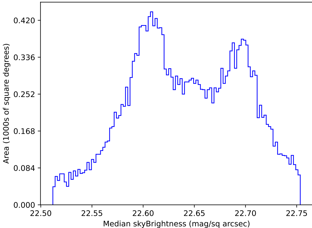
too_elab_r256_d2_gz_v3.4_10yrs All sky u band: Median skyBrightness
