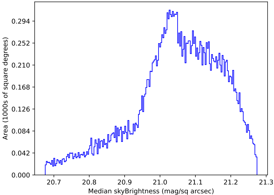
too_elab_r256_d2_gz_v3.4_10yrs All sky r band: Median skyBrightness
