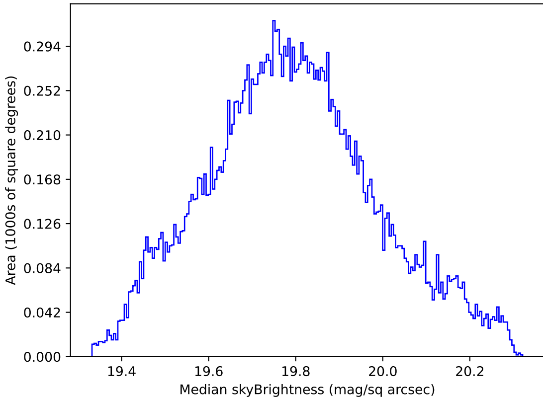
too_elab_r256_d2_gz_v3.4_10yrs All sky all bands: Median skyBrightness
