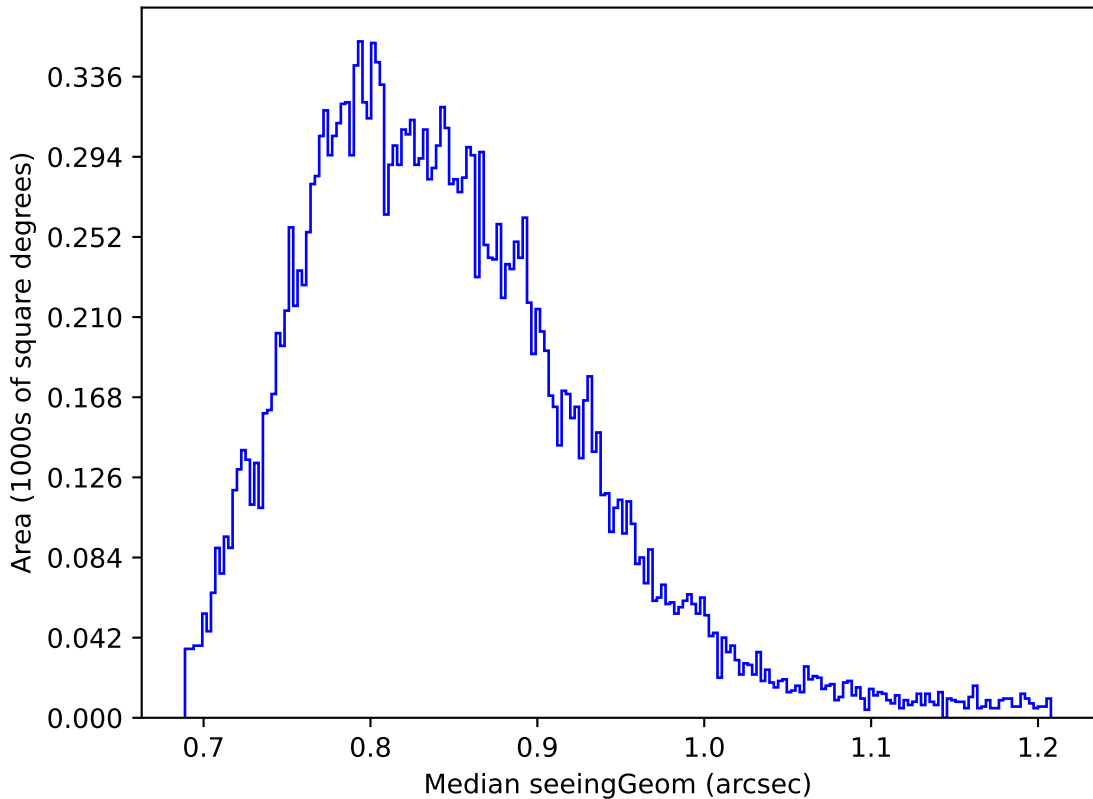
too_elab_r256_d2_gz_v3.4_10yrs Yr 1 y band: Median seeingGeom
