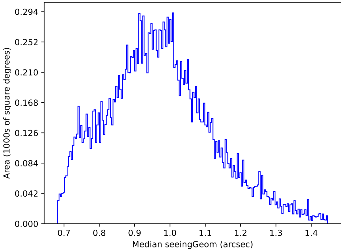
too_elab_r256_d2_gz_v3.4_10yrs Yr 1 u band: Median seeingGeom
