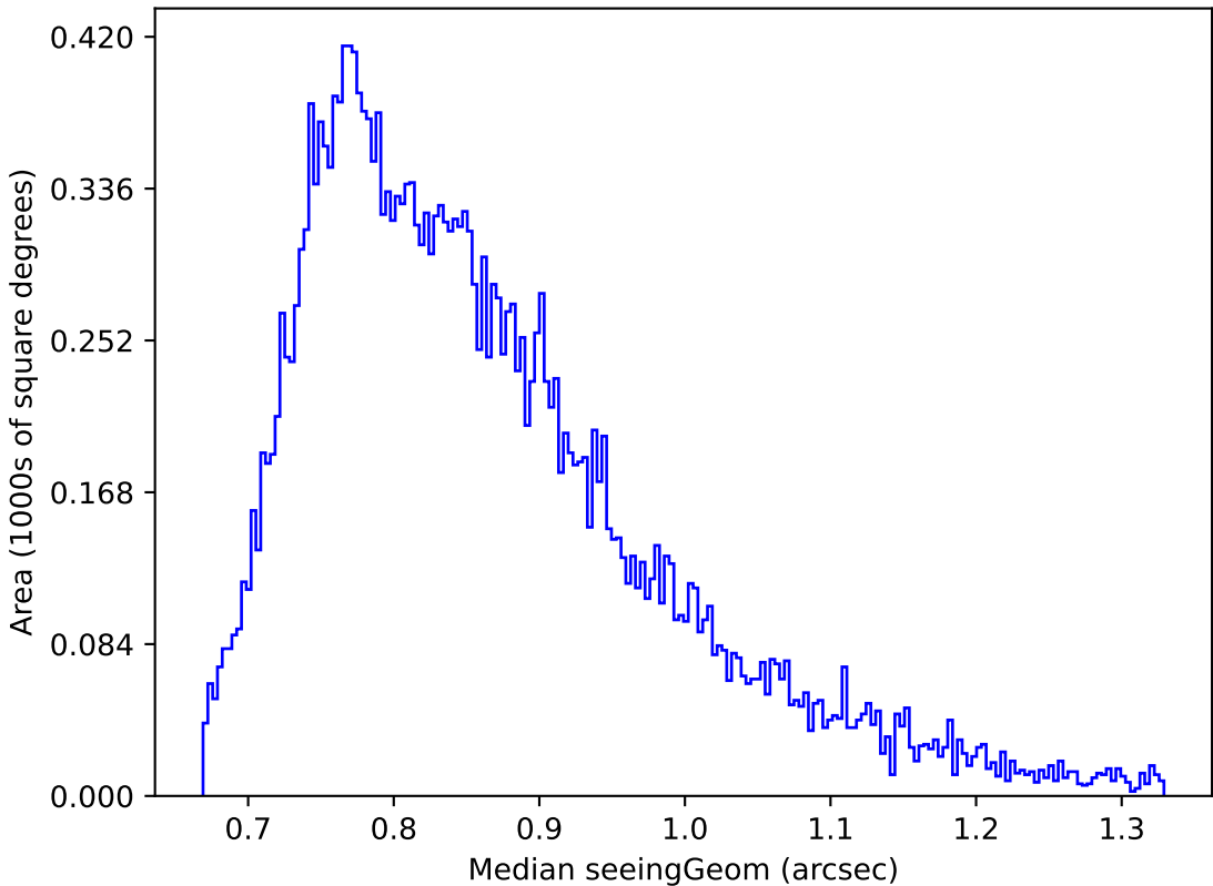
too_elab_r256_d2_gz_v3.4_10yrs Yr 1 r band: Median seeingGeom
