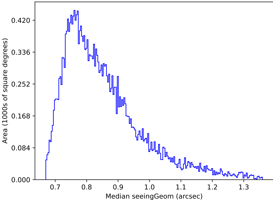
too_elab_r256_d2_gz_v3.4_10yrs Yr 1 i band: Median seeingGeom
