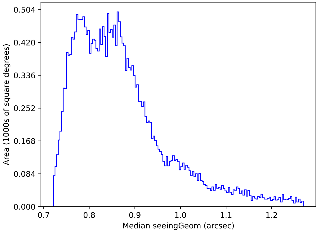
too_elab_r256_d2_gz_v3.4_10yrs Yr 1 all bands: Median seeingGeom
