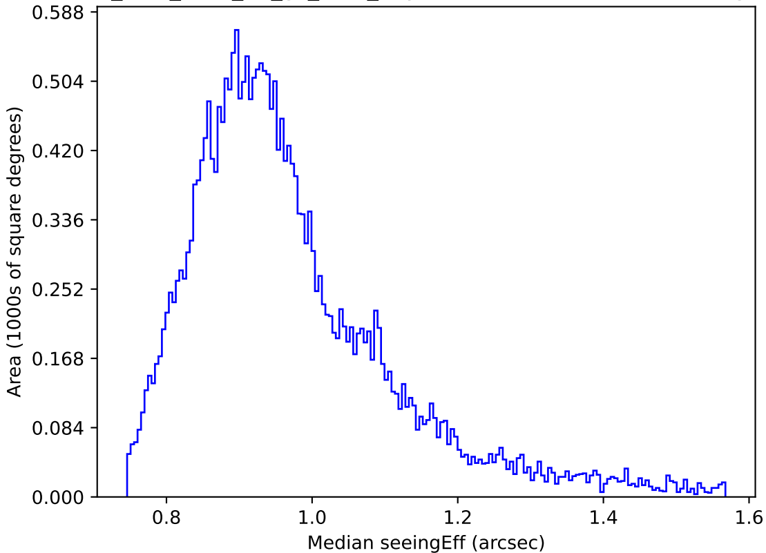
too_elab_r256_d2_gz_v3.4_10yrs Yr 1 z band: Median seeingEff
