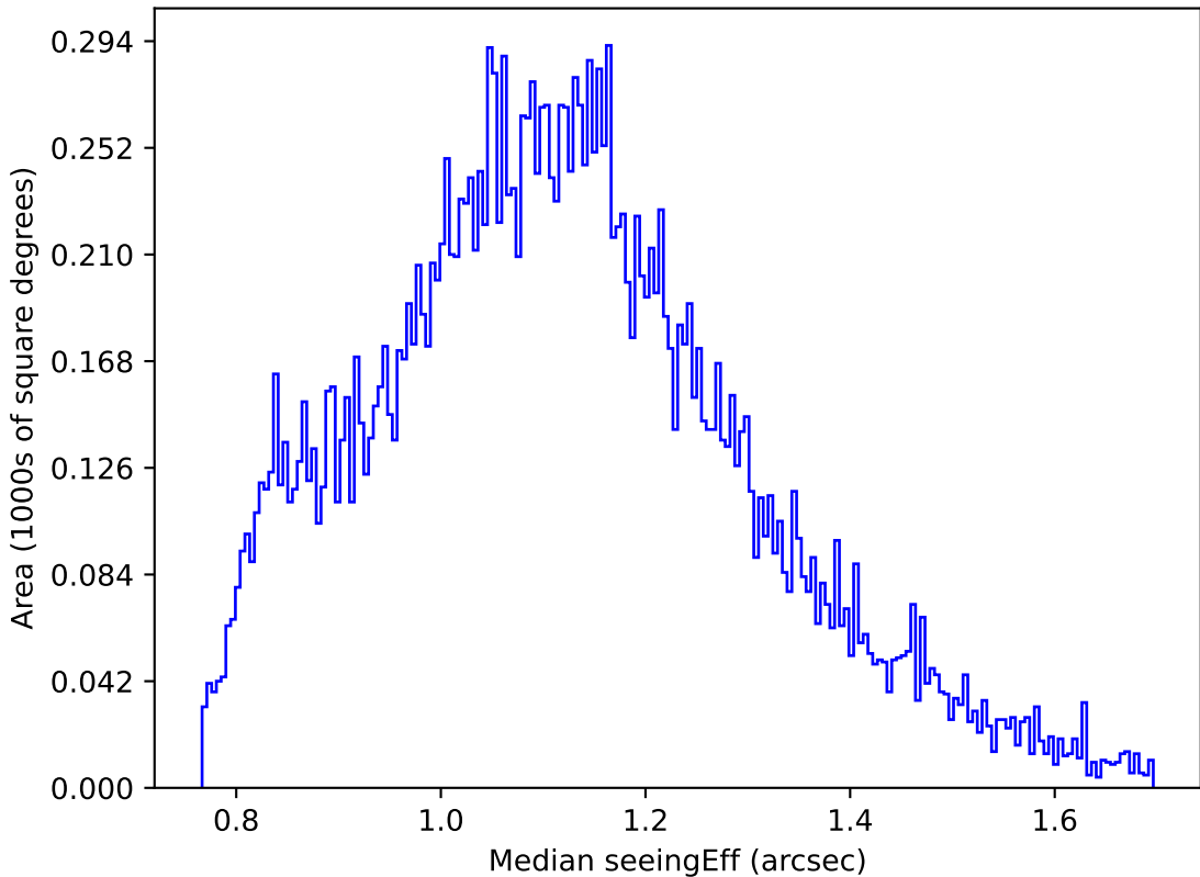
too_elab_r256_d2_gz_v3.4_10yrs Yr 1 u band: Median seeingEff
