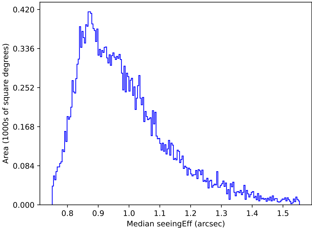
too_elab_r256_d2_gz_v3.4_10yrs Yr 1 r band: Median seeingEff
