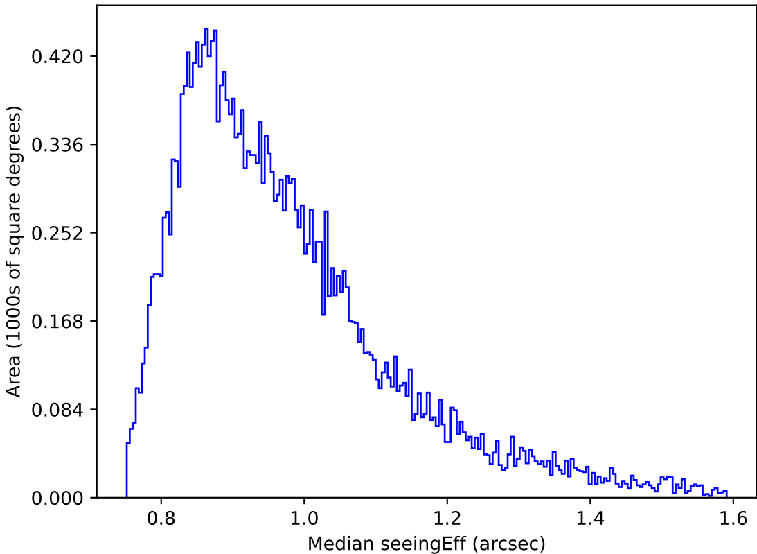
too_elab_r256_d2_gz_v3.4_10yrs Yr 1 i band: Median seeingEff
