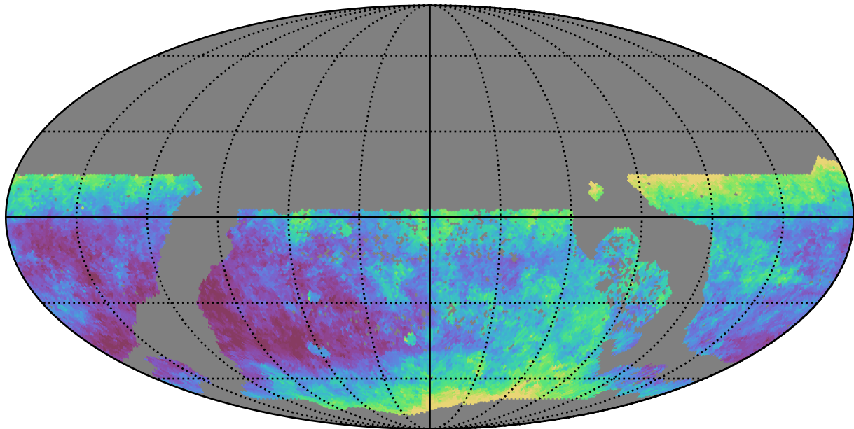
too_elab_r256_d2_gz_v3.4_10yrs WFD z band: Median seeingEff
